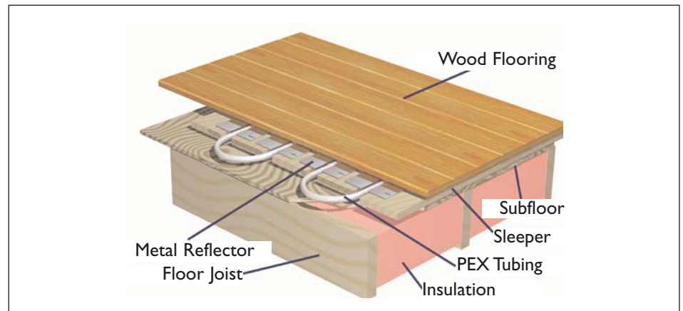
Figure 2. Suspended in subfloor. Image courtesy of Wirsbo Co.
